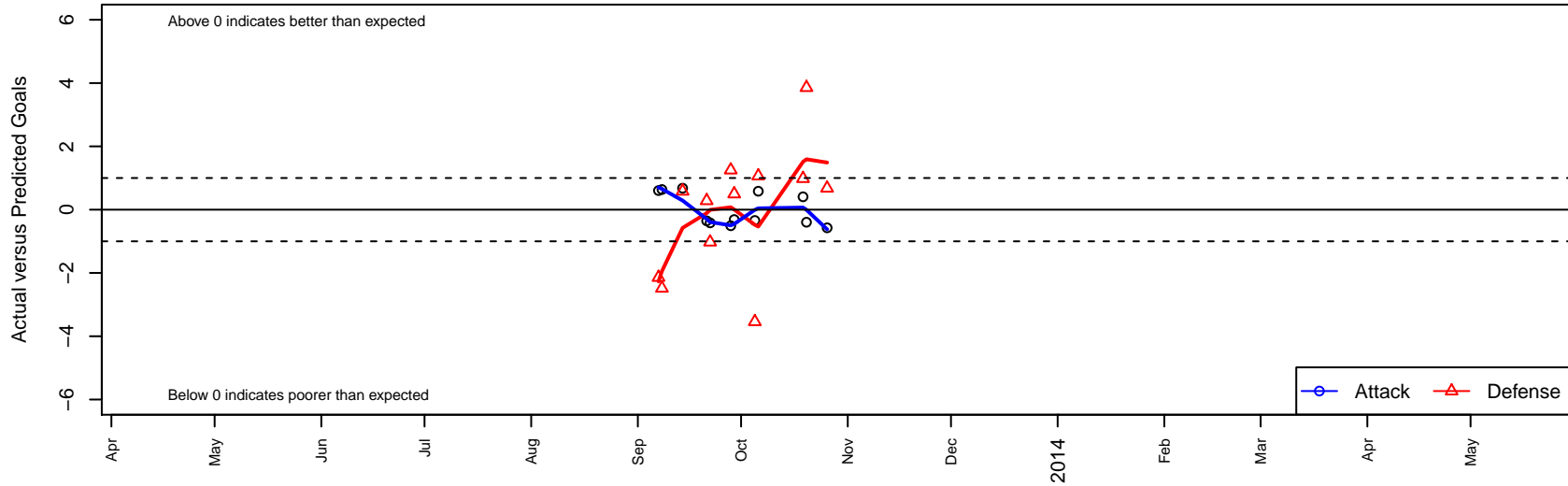
Foothills SC Celtic White B02 Dots are actual minus expected GF (blue circles) and GA (red triangles). Blue line is smoothed change in attack strength. Red is smoothed change in defense strength.
